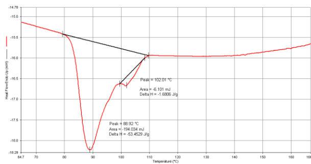
Figure S6. DSC thermograms of S-CBCONH5CB upon several heating and cooling cycles, m = 3.63 mg, 10\text{ }^{\circ}\text{C}/\text{min}
